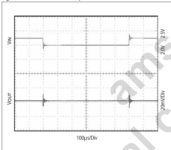
Figure 17. Line Transient Response; I_{OUT} = 350mA
