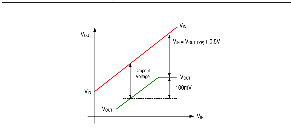
Figure 21. Graphical Representation of Dropout Voltage
