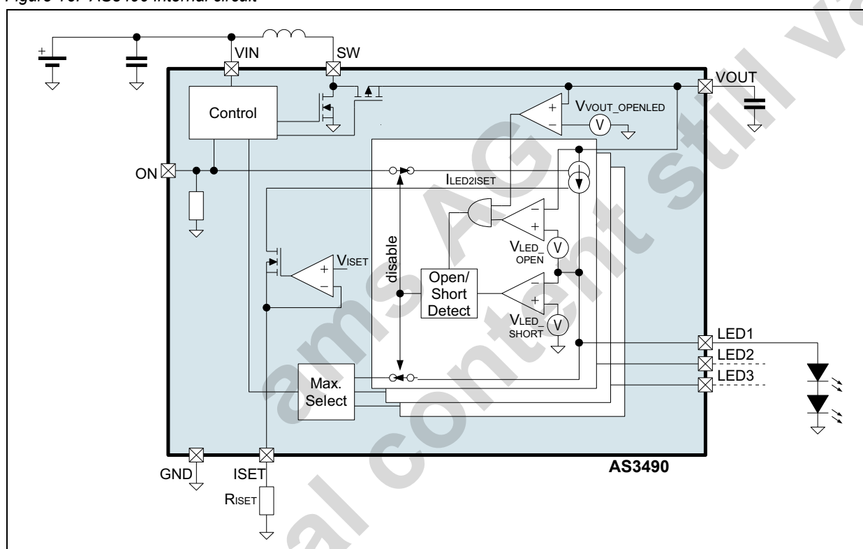
Figure 16. AS3490 internal circuit
