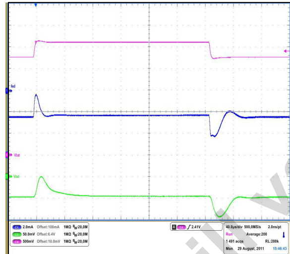
Figure 10. VIN line transient 10µs (ILOAD=100mA)
