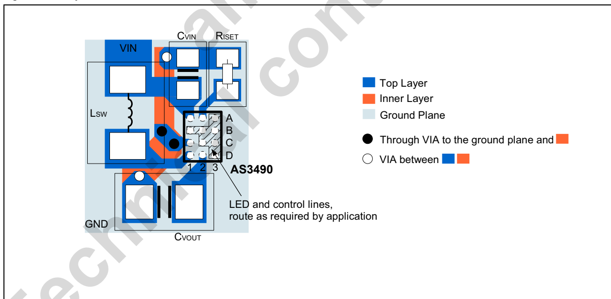
Figure 20. Layout recommendation
