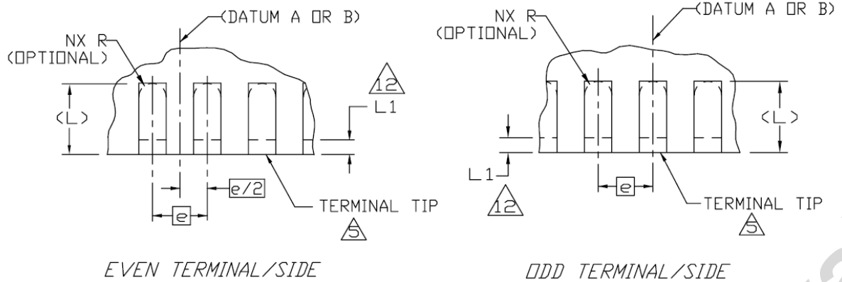
DETAIL B
