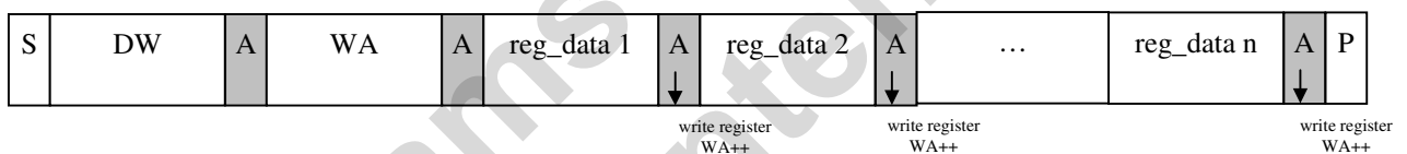
Figure 2 – I 2 C Page-Write:
