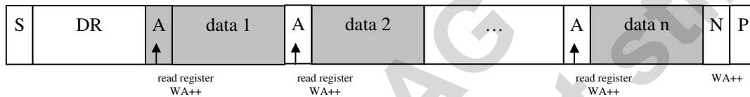
Figure 5 – I^2C Current-Address-Read:
