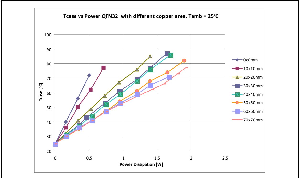
Figure 11: TCASE vs. Power with Different Copper Area @ T_{AMB} = 25^{\circ}C
