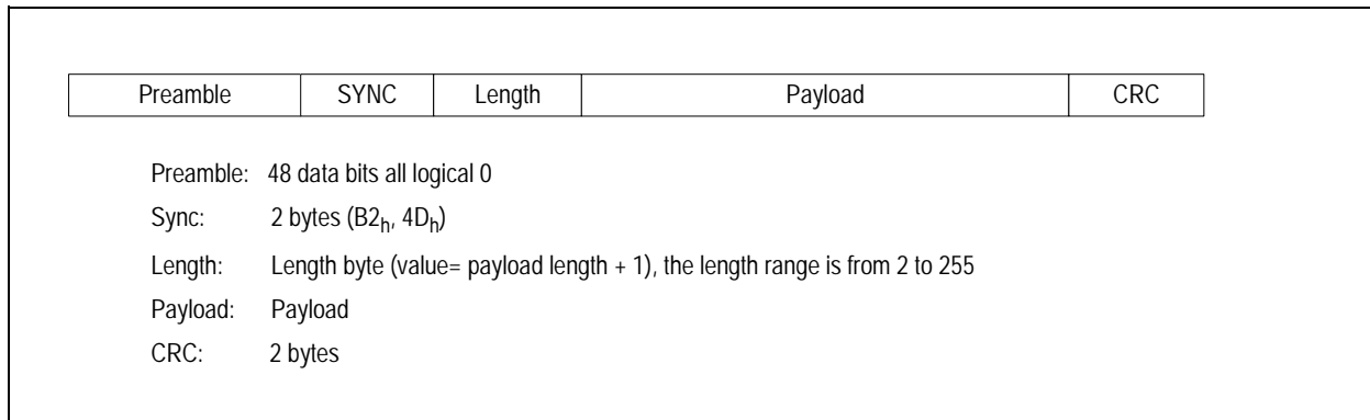
Figure 124: FeliCa Frame Format
