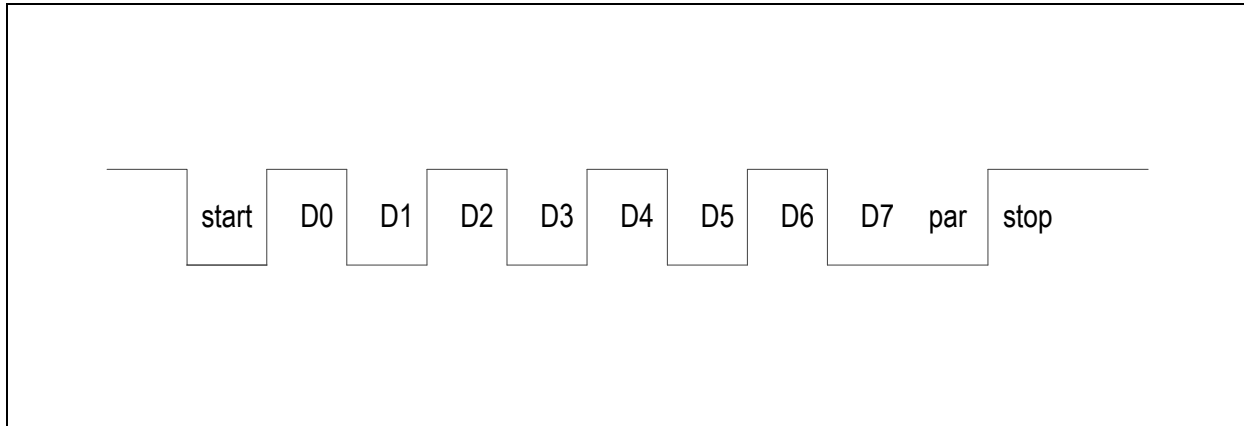
Figure 14. Synchronization Frame
