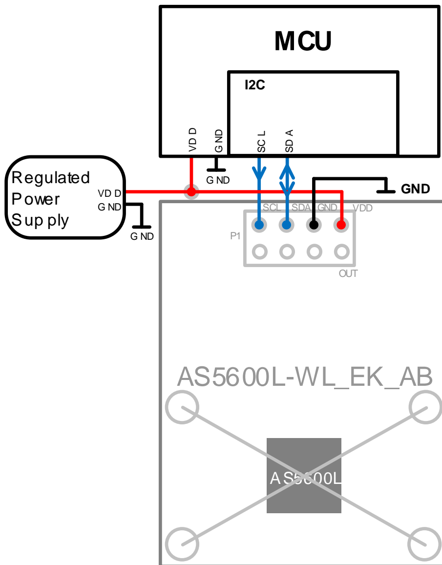
Figure 5: I2C Mode
