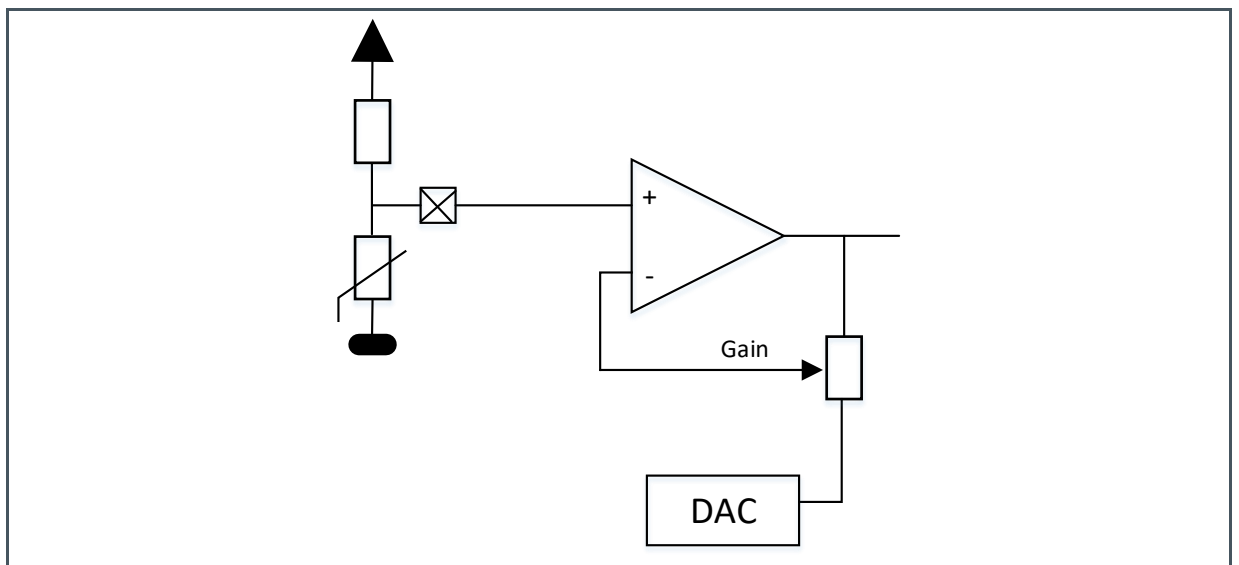
Figure 114: Non Inverting Amplifier with Offset and Input Voltage Divider (Temperature Sensor)
