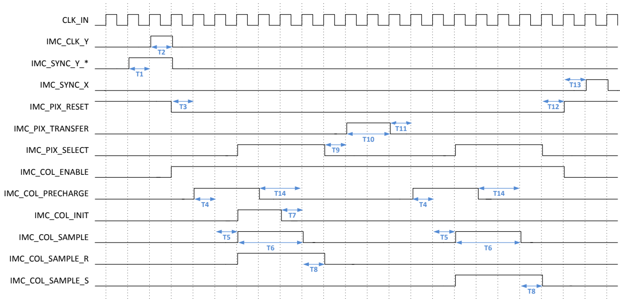
Figure 9: Timing diagram
