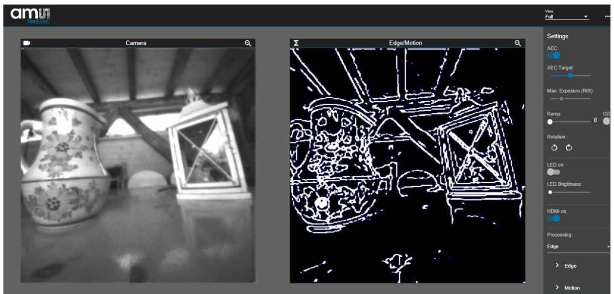
Figure 4: NanoBerry GUI
