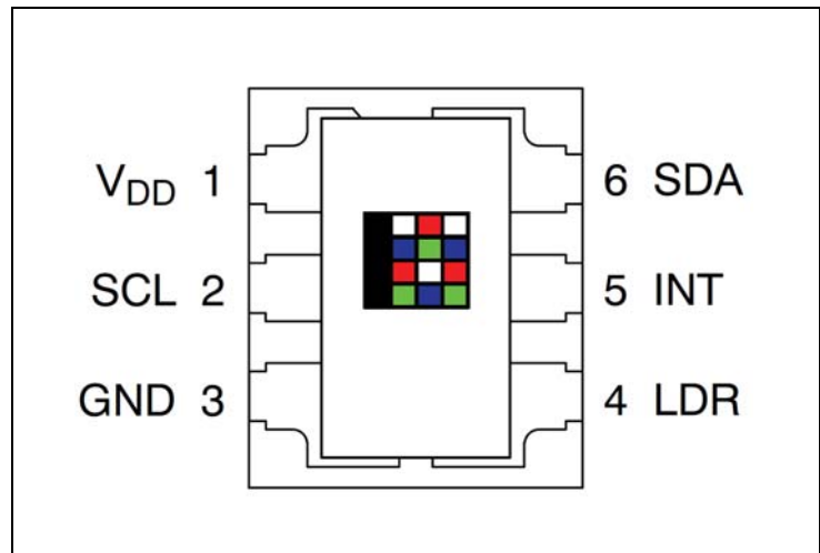
Figure 3: Pin Diagram
