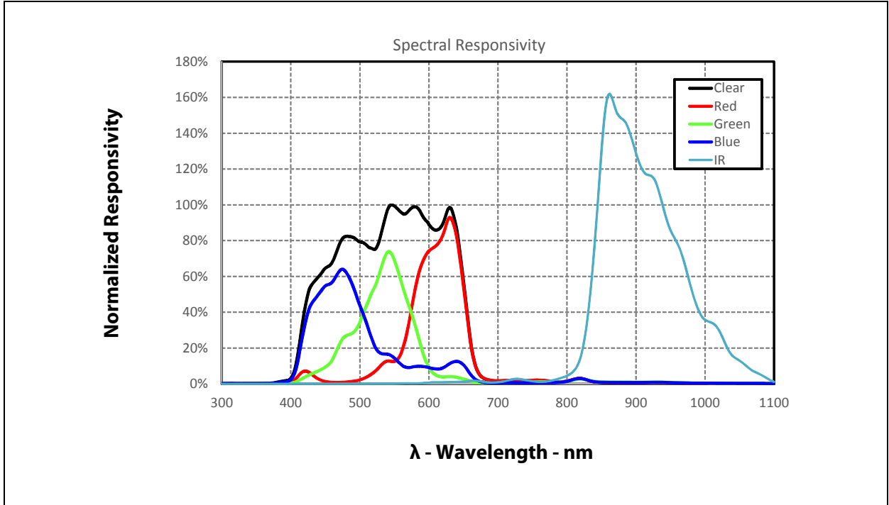
Figure 16: Spectral Responsivity
