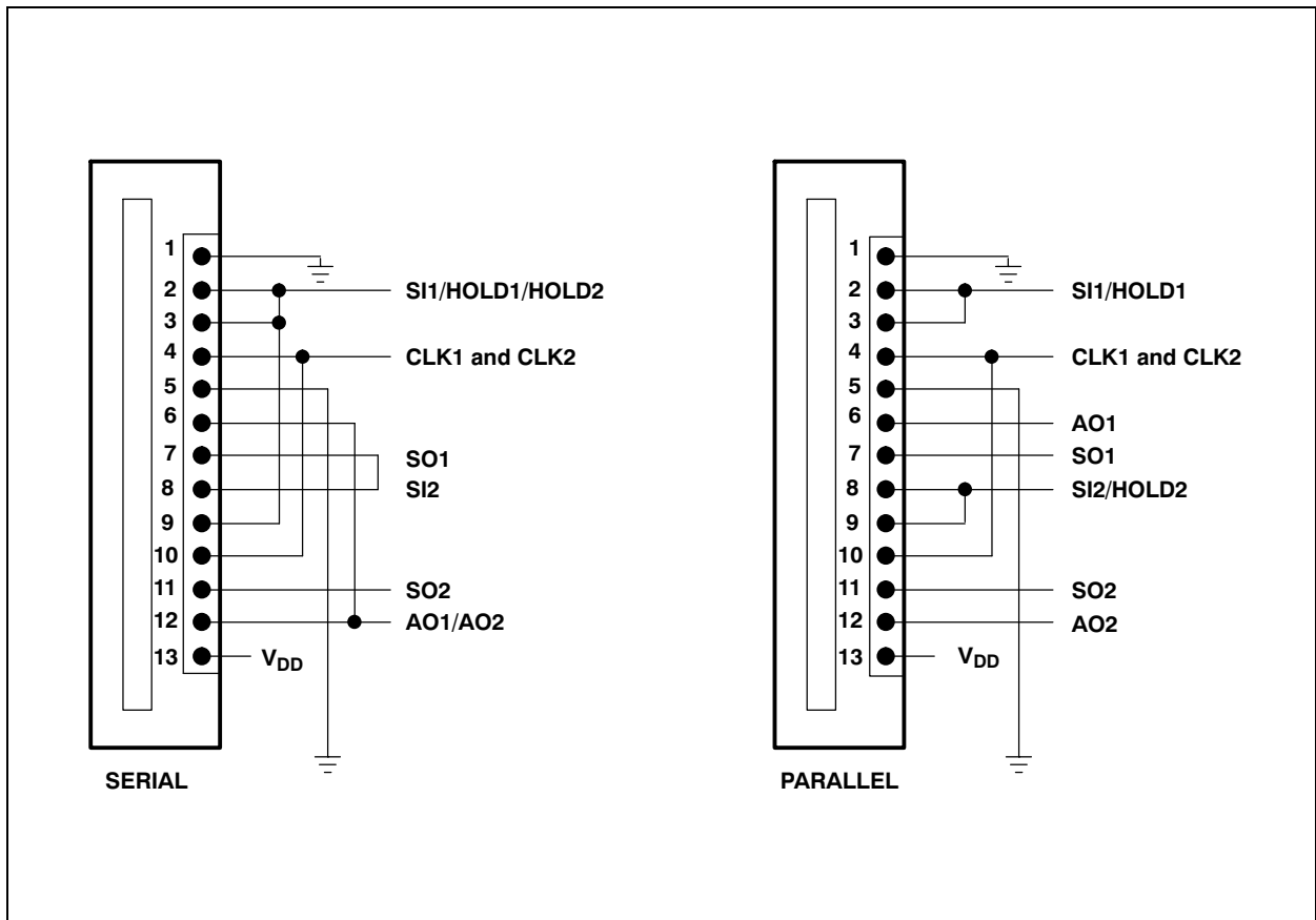
Figure 18: Operational Connections
