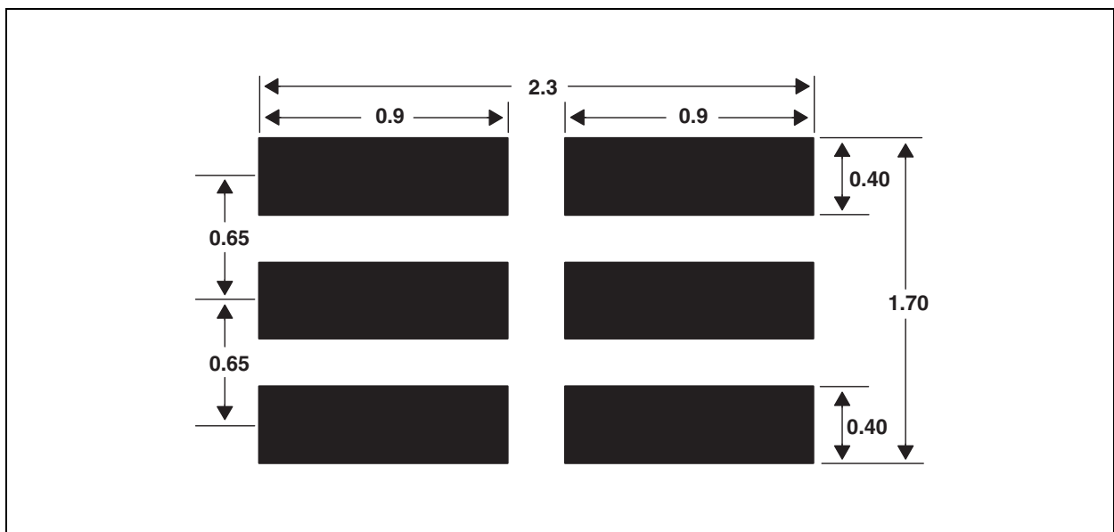
Figure 33: Suggested FN Package PCB Layout
