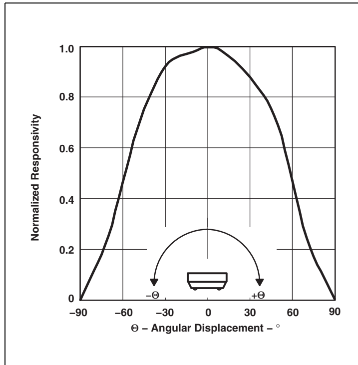
Figure 14: Normalized Responsivity vs. Angular Displacement
