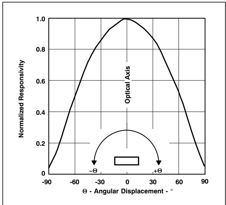
Figure 12: Normalized Responsivity vs. Angular Displacement - CL Package
