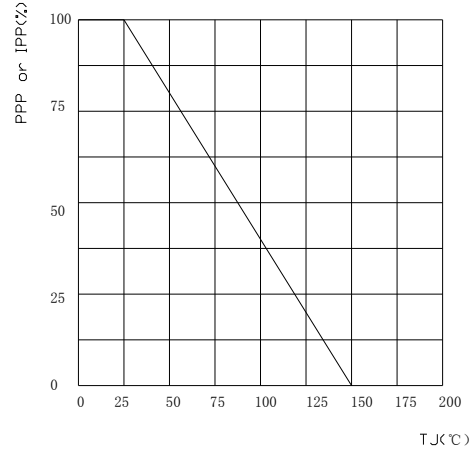
FIG2: Pulse Power or Current vs.Initial Junction Temperature
