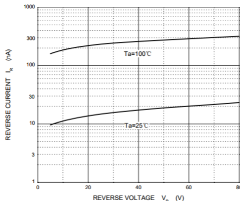
Reverse Characteristics
