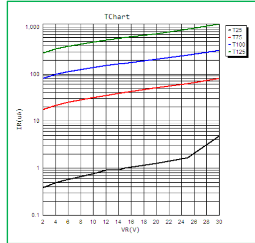
Reverse Characteristics
