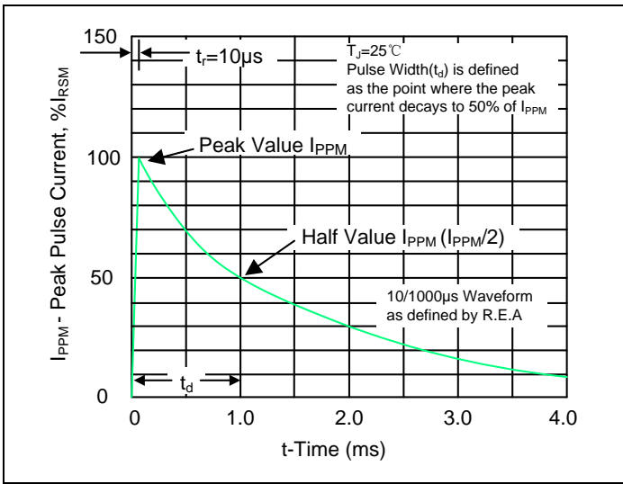
Figure 3. Pulse Waveform
