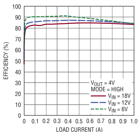
Figure 5. Buck Efficiency
