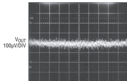
C_{OUT} = 10\mu F 1ms/DIV 1761 G48 I_L = 100mA
