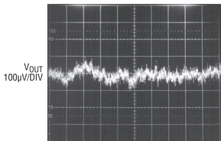
C_{OUT} = 10\mu F 1ms/DIV 1761 G47 I_L = 100mA
