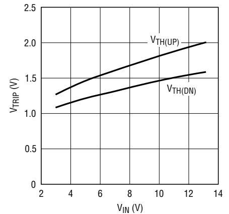
\overline{\text{SHDN}} Input Voltage Thresholds vs V_{\text{IN}}
