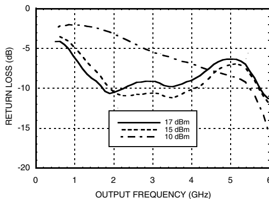
Output Return Loss with 2.5 GHz Input
