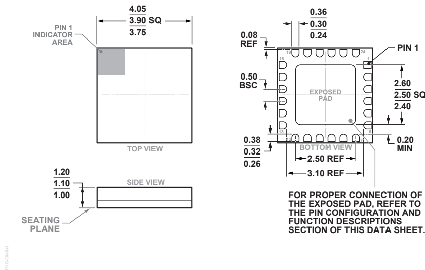
24-Terminal Ceramic Leadless Chip Carrier [LCC] (E-24-2)
