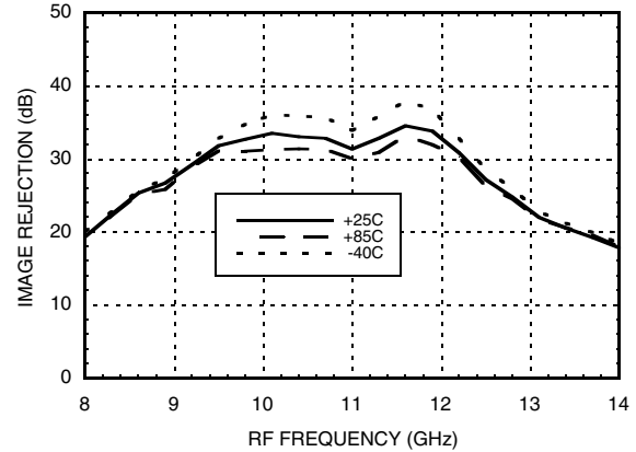
Image Rejection vs. Temperature
