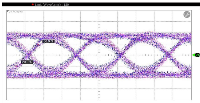
40 Gbps Single-Ended Output Eye Diagram
