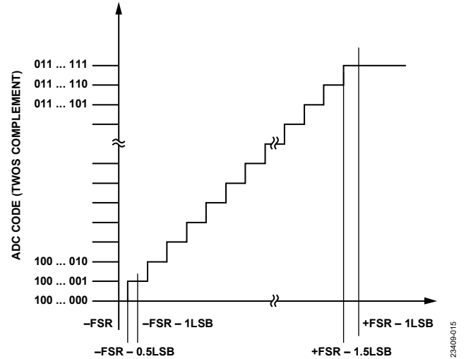
Figure 33. ADC Ideal Transfer Function (FSR = Full-Scale Range)
