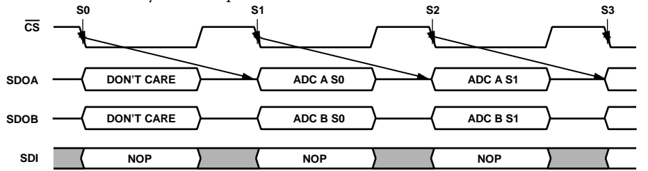
Figure 41. Reading Conversion Results: 2-Wire Mode
