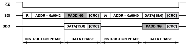
Figure 92. Single Instruction Mode SPI Frame, MB_STRICT = 1, Ascending Address
