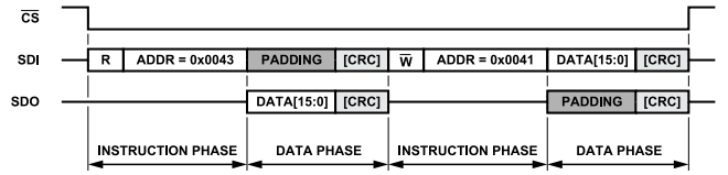
Figure 91. Single Instruction Mode SPI Frame, MB_STRICT = 1, Descending Address
