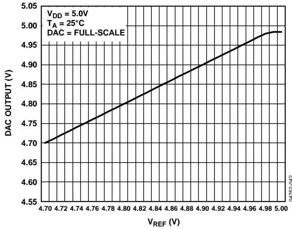
Figure 28. Typical Output Voltage vs. Reference Voltage
