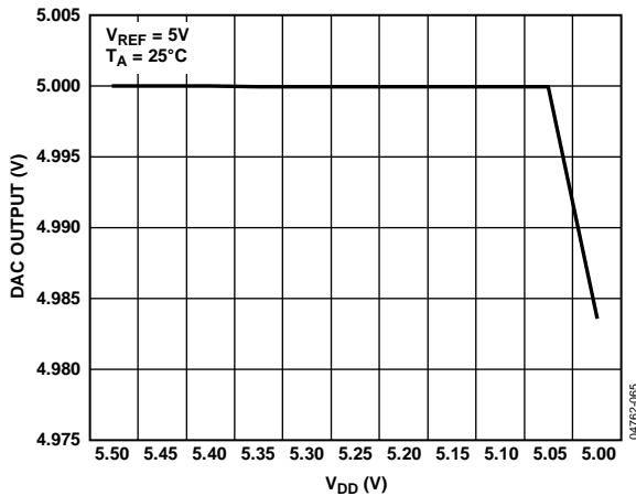
Figure 29. Typical Output Voltage vs. Supply Voltage
