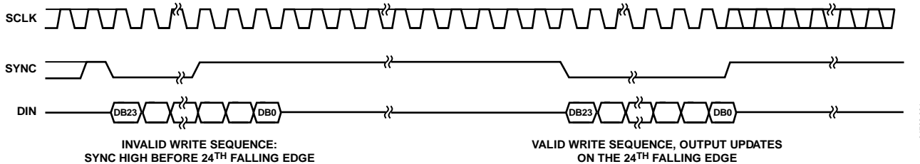
Figure 40. \overline{\text{SYNC}} Interrupt Facility
