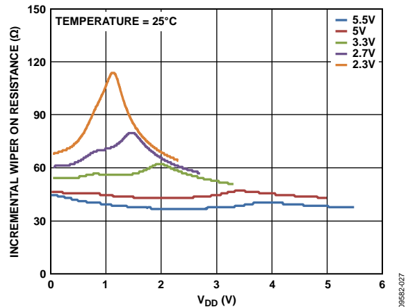
Figure 27. Incremental Wiper On Resistance vs. V_{DD}
