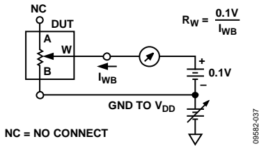
Figure 37. Wiper Resistance
