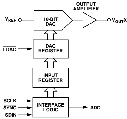
Figure 47. Simplified Diagram of Input Loading Circuitry for a Single DAC
