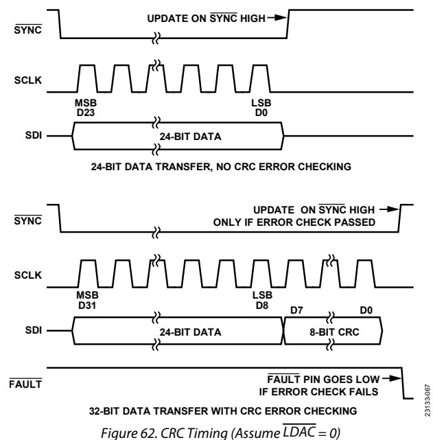
Figure 62. CRC Timing (Assume \overline{LDAC} = 0 )
