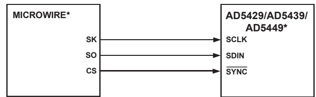
Figure 53. MICROWIRE-to-AD5429/AD5439/AD5449 Interface
