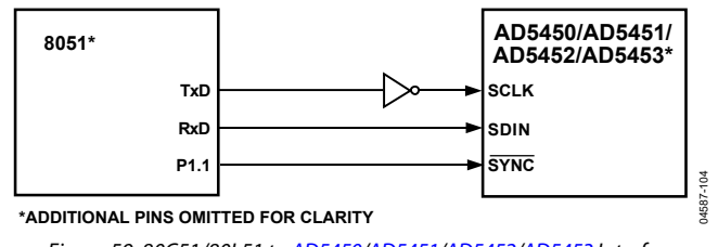
Figure 59. 80C51/80L51 to AD5450/AD5451/AD5452/AD5453 Interface
