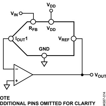
NOTE ADDITIONAL PINS OMITTED FOR CLARITY Figure 48. Current Steering DAC Used as a Divider or Programmable Gain Element
