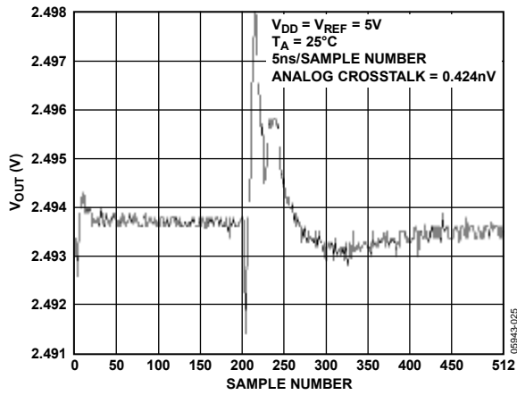
Figure 24. Analog Crosstalk
