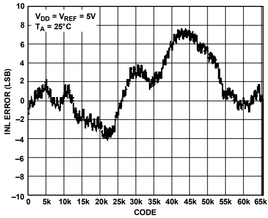
Figure 4. INL—External Reference
