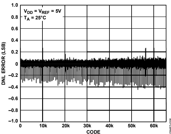
Figure 6. DNL—External Reference
