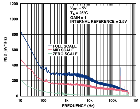
Figure 46. Noise Spectral Density (NSD)
