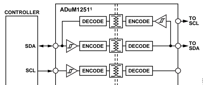
Figure 69. Isolated Interface
