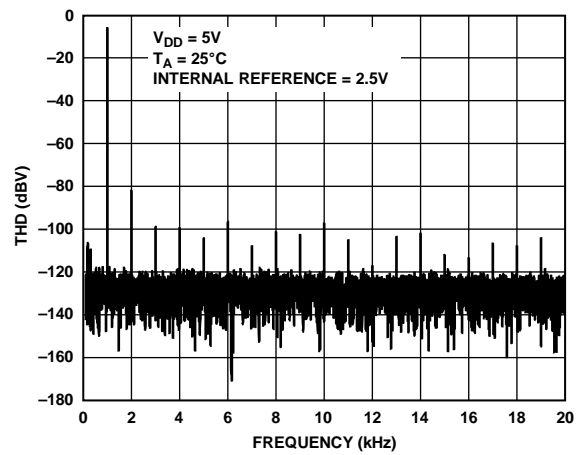
Figure 47. THD at 1 kHz
