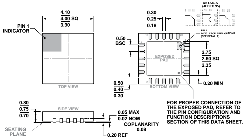
COMPLIANT TO JEDEC STANDARDS MO-220-WGGD-11. Figure 54. 20-Lead Lead Frame Chip Scale Package [LFCSPP] 4 mm x 4 mm Body and 0.75 mm Package Height (CP-20-8) Dimensions shown in millimeters
