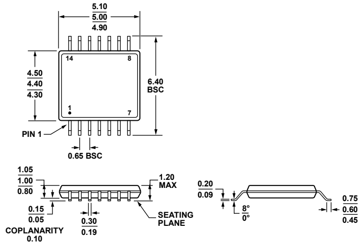
COMPLIANT TO JEDEC STANDARDS MO-153-AB-1 Figure 51. 14-Lead Thin Shrink Small Outline Package [TSSOP] (RU-14) Dimensions shown in millimeters
