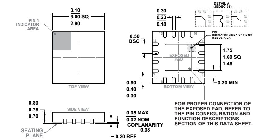
Figure 63. 16-Lead Lead Frame Chip Scale Package [LFCSP] 3 mm × 3 mm Body and 0.75 mm Package Height (CP-16-22)
