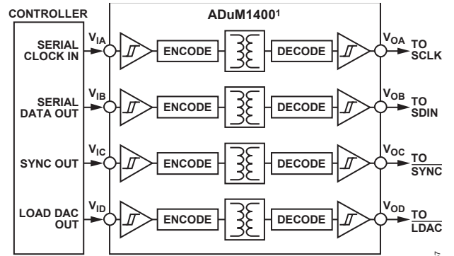
Figure 62. Isolated Interface
