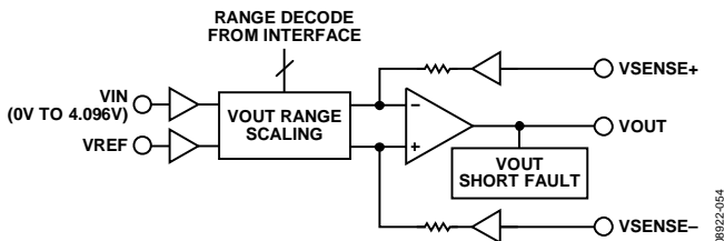
Figure 52. Voltage Output
