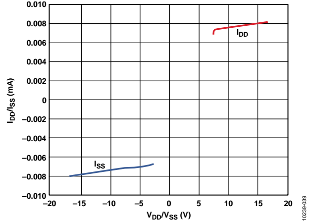
Figure 38. Power Supply Currents vs. Power Supply Voltages
