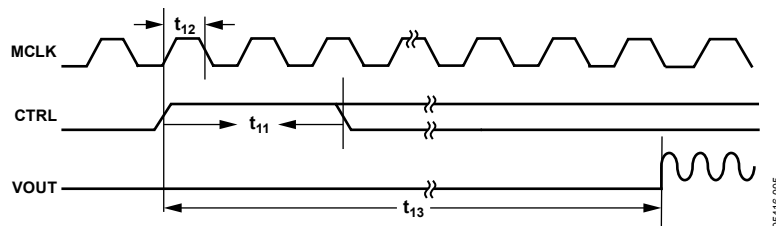
Figure 5. CTRL Timing
