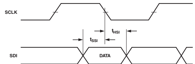
Figure 46. Serial Input Data Timing Requirements
