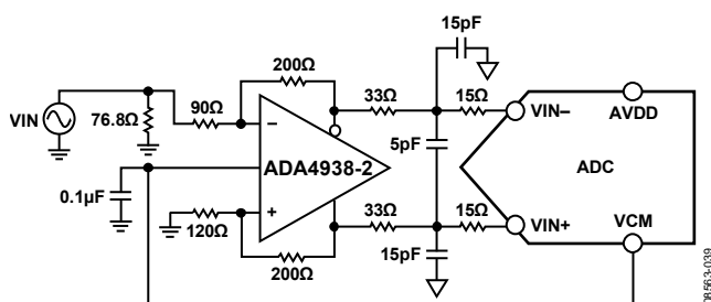
Figure 30. Differential Input Configuration Using the ADA4938-2
