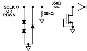
Figure 32. Equivalent SCLK and PDWN Input Circuit
