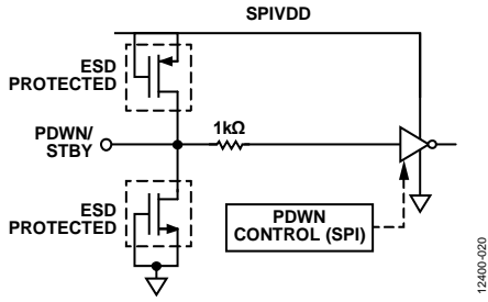
Figure 72. PDWN/STBY Input
