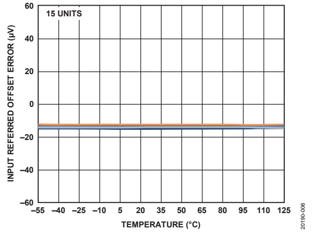
Figure 6. Input Referred Offset Error vs. Temperature (Gain = 16, Full Power Mode)
