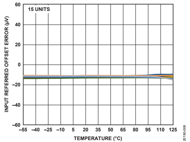
Figure 8. Input Referred Offset Error vs. Temperature (Gain = 16, Low Power Mode)
