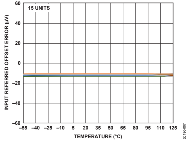
Figure 7. Input Referred Offset Error vs. Temperature (Gain = 16, Mid Power Mode)
