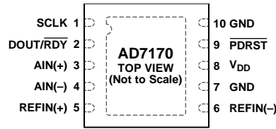
Figure 5. Pin Configuration
